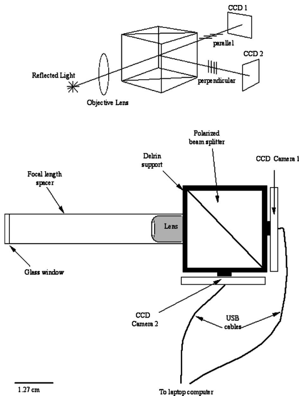
Fig. 1 Main components of the handheld polarization system. The top figure shows the main components of the system: polarizing beam-splitter cube, two CCD cameras, and an objective lens. The bottom figure is a top view of the setup showing the CCD cameras attached to a Delrin support enclosing the beamsplitter cube.
