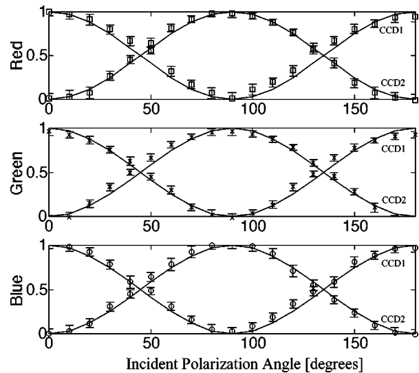
Fig. 3 Performance test for polarized optics. The x axis denotes the angle of orientation of the linear polarization of the light source (0 denotes parallel to horizontal axis of beamsplitter). The y axis denotes the detected intensity for the red, green and blue channels of the two cameras (at x axis equal to 0, the parallel CCD 1 camera sees maximum light and the perpendicular CCD 2 camera sees minimum light).
