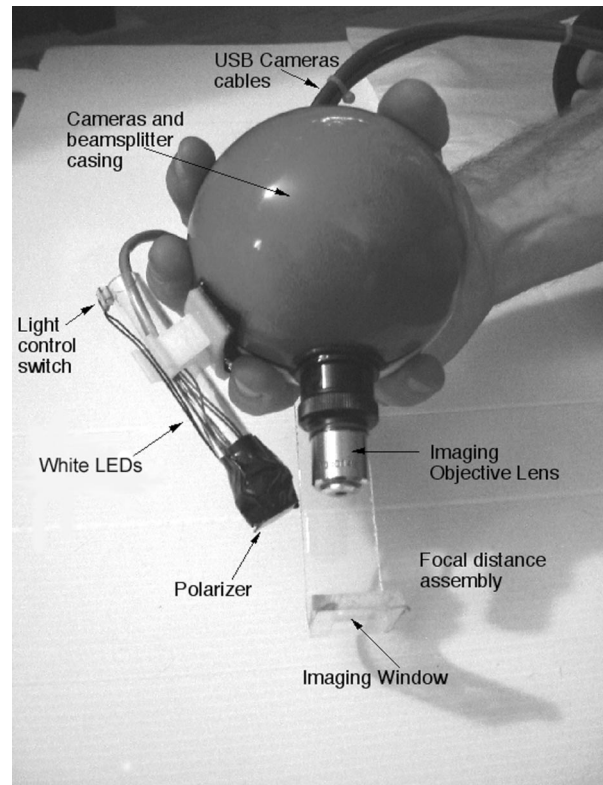
Fig. 2 Clinical handheld polarization system; spherical casing protects the main components and makes the prototype easy to hold with one hand.
