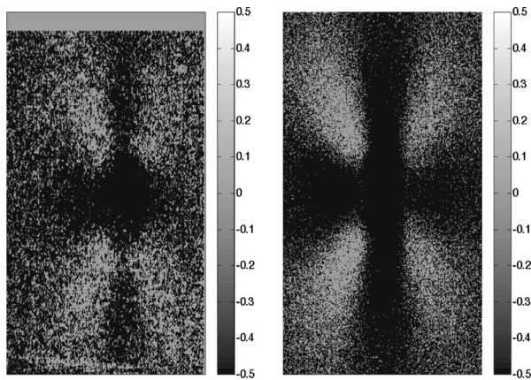
Fig. 4 Monte Carlo model and experimental results of a 633-nm-wavelength laser beam scattering from a solution of 2- \mu\text{m} microspheres in water. On the left is the plot of the experimental polarized image, and on the right is the corresponding plot of the Monte Carlo model.
