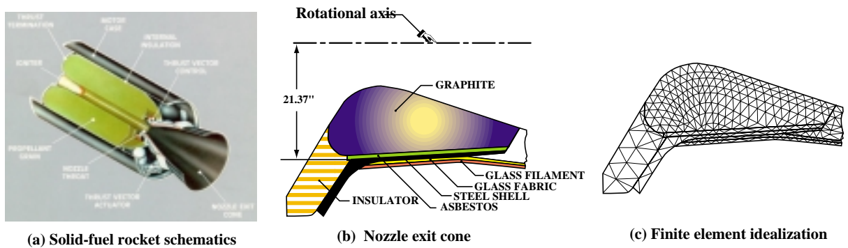
FIGURE 10.3. Axisymmetric FE analysis of a typical rocket nozzle (carried out by E. L. Wilson at Aerojet Corporation, circa 1963). Figure from paper cited in footnote 1.
