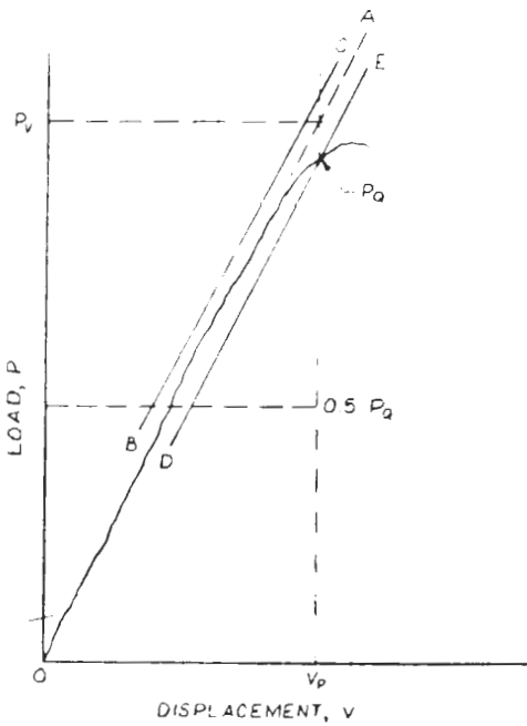
FIG. A7.1 Special Requirements for Analysis of Load Versus Displacement Records (5 % Secant Line Not Shown)
