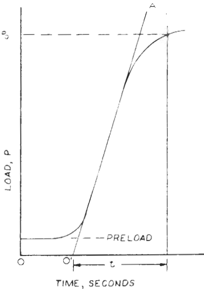
FIG. A7.2 Determination of Test Time From Load Versus Time Record
