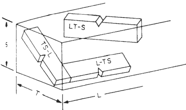
FIG. 2 Crack Plane Orientation Code for Rectangular Sections Where Specimens are Tilted with Respect to the Reference Directions
