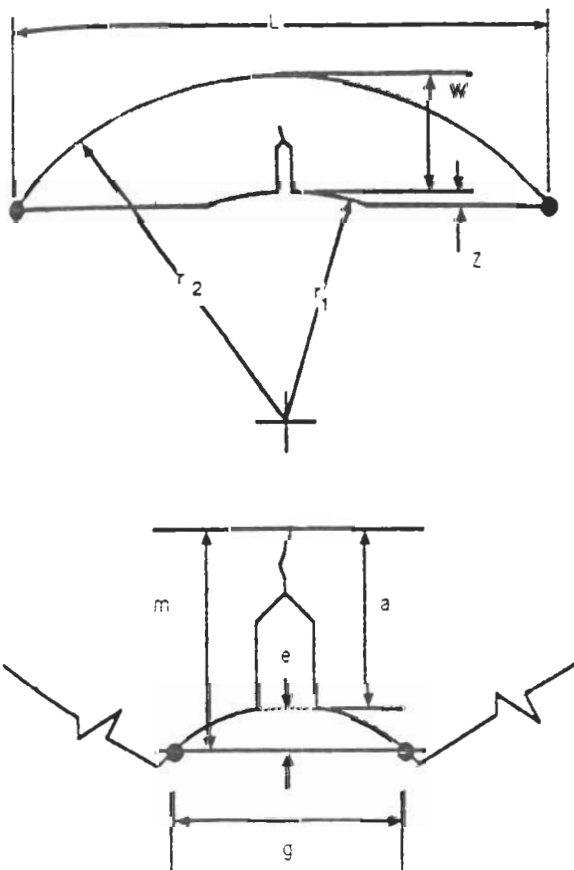
FIG. A9.2 Measurement of Outer Radius ( r_2 ) and Crack Length for the Arc-Shaped Bend Specimen (see A9.4.1.1)
