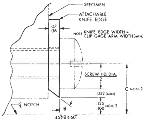
FIG. 5 Example of Integral Knife Edge Design
