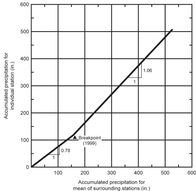
Figure 2.3 Double-mass curve for Example 2.3.
