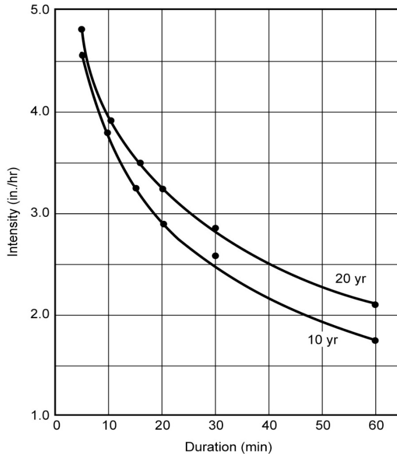
Figure 2.6 Intensity-duration-frequency curve.
