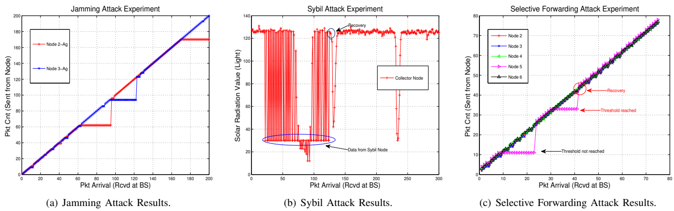
Fig. 5: Attack Experiments.
