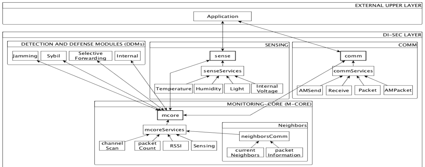
Fig. 1: Di-Sec Architecture.
