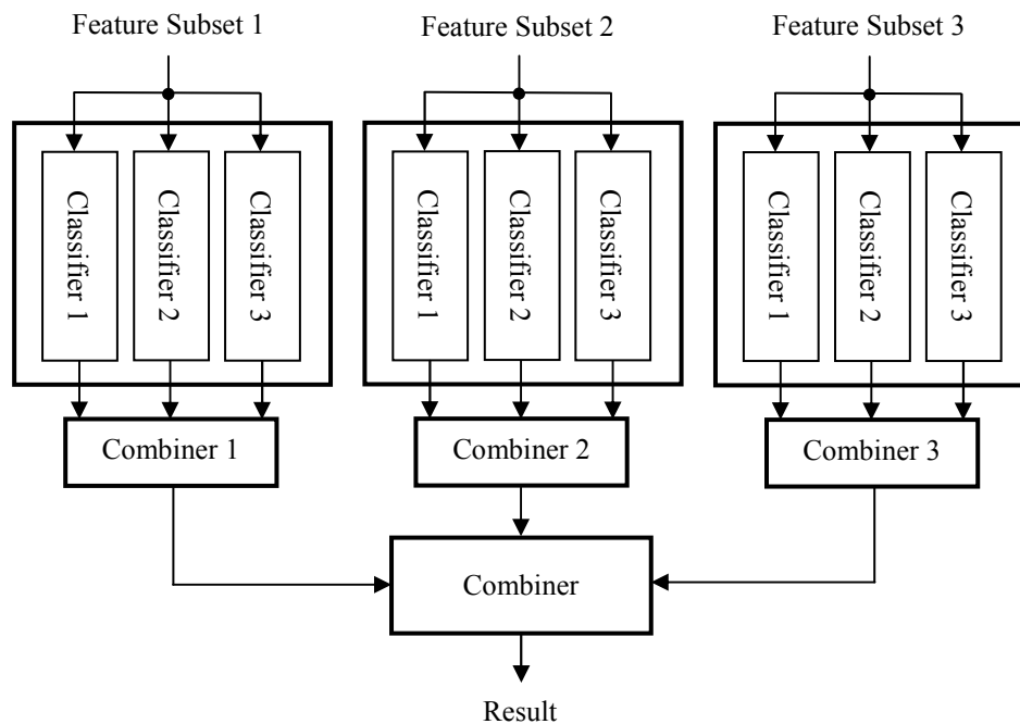
Figure 1. Topologies of Proposed Intrusion Detection System
