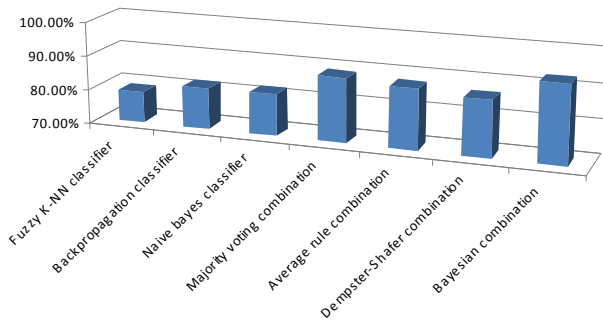
Figure 2. CRs of Three Classifiers Using Full Feature Set and Approaches Using Four Different Combination Methods
