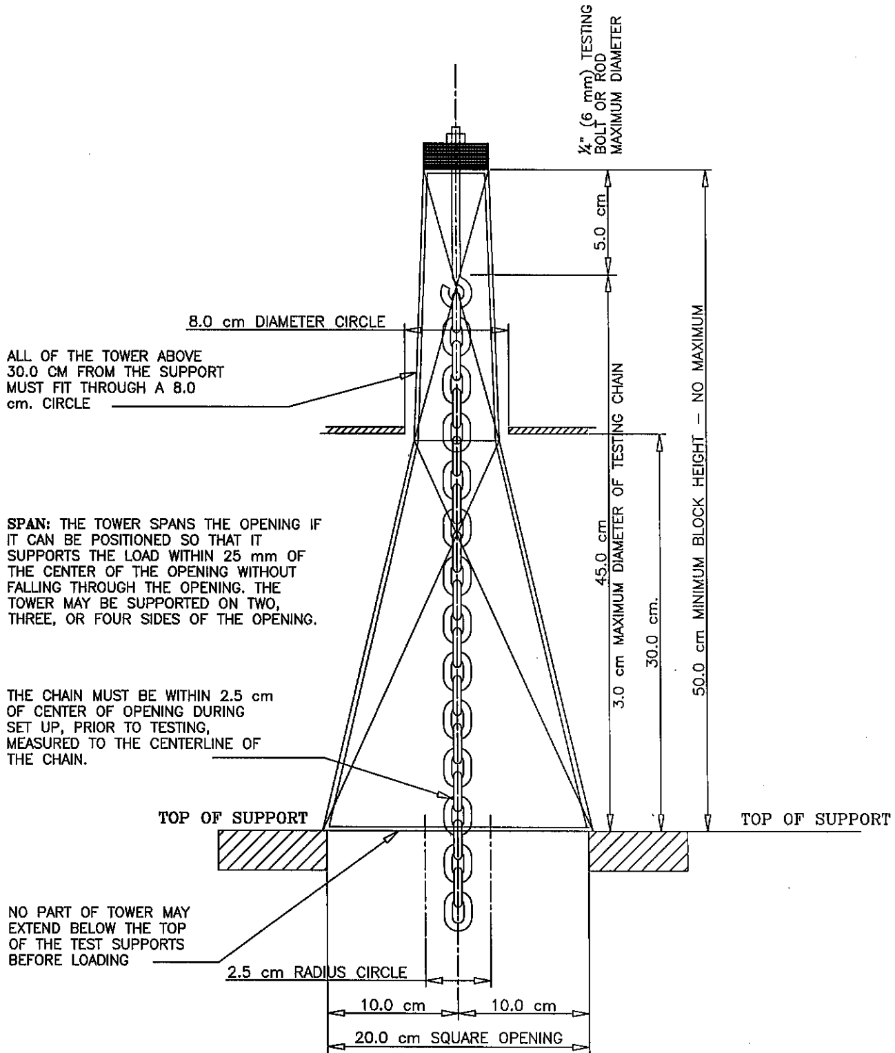
SIDE VIEW
